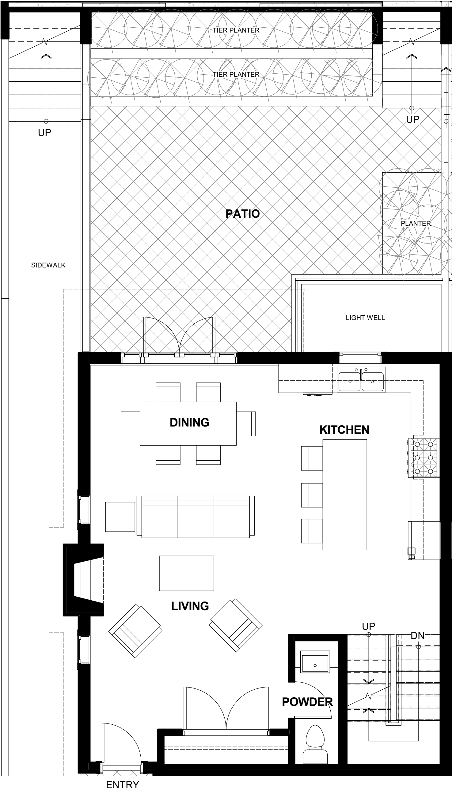
MAIN - D Scale 1/4" = 1'- 0"
