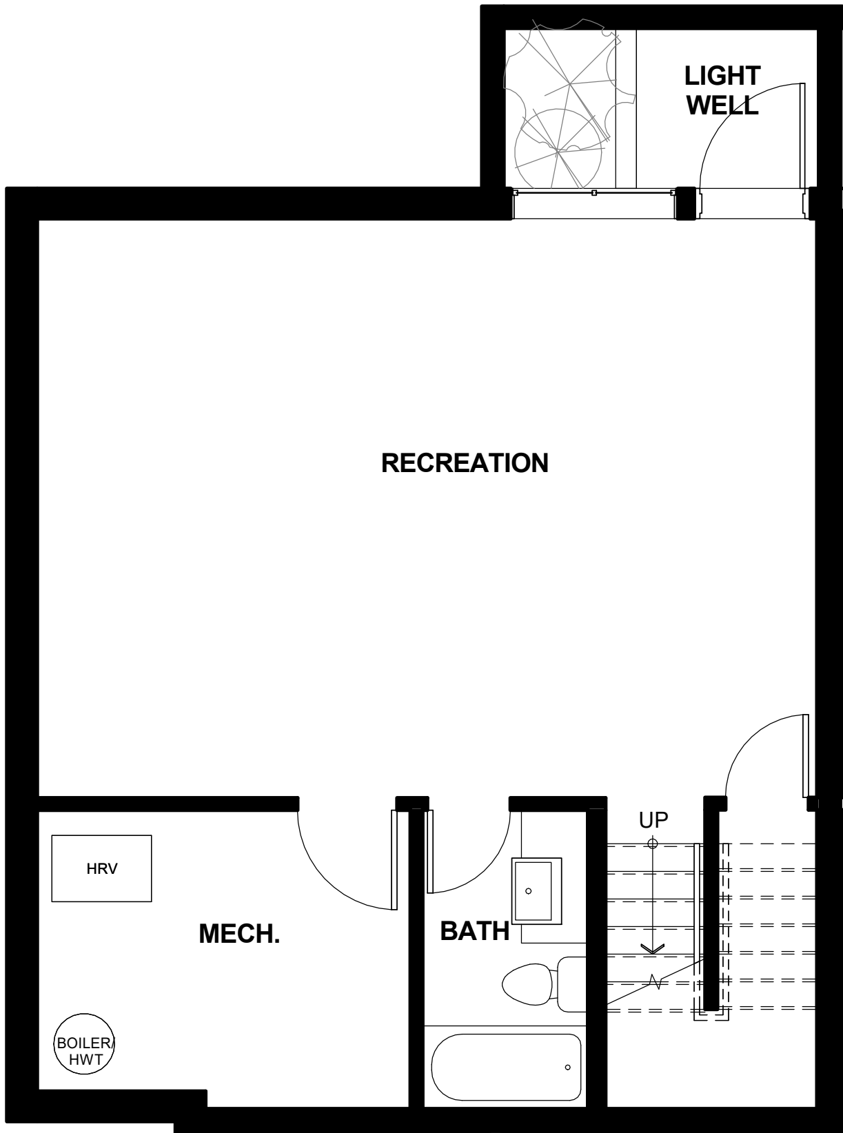
BASEMENT - D Scale 1/4" = 1'- 0"
