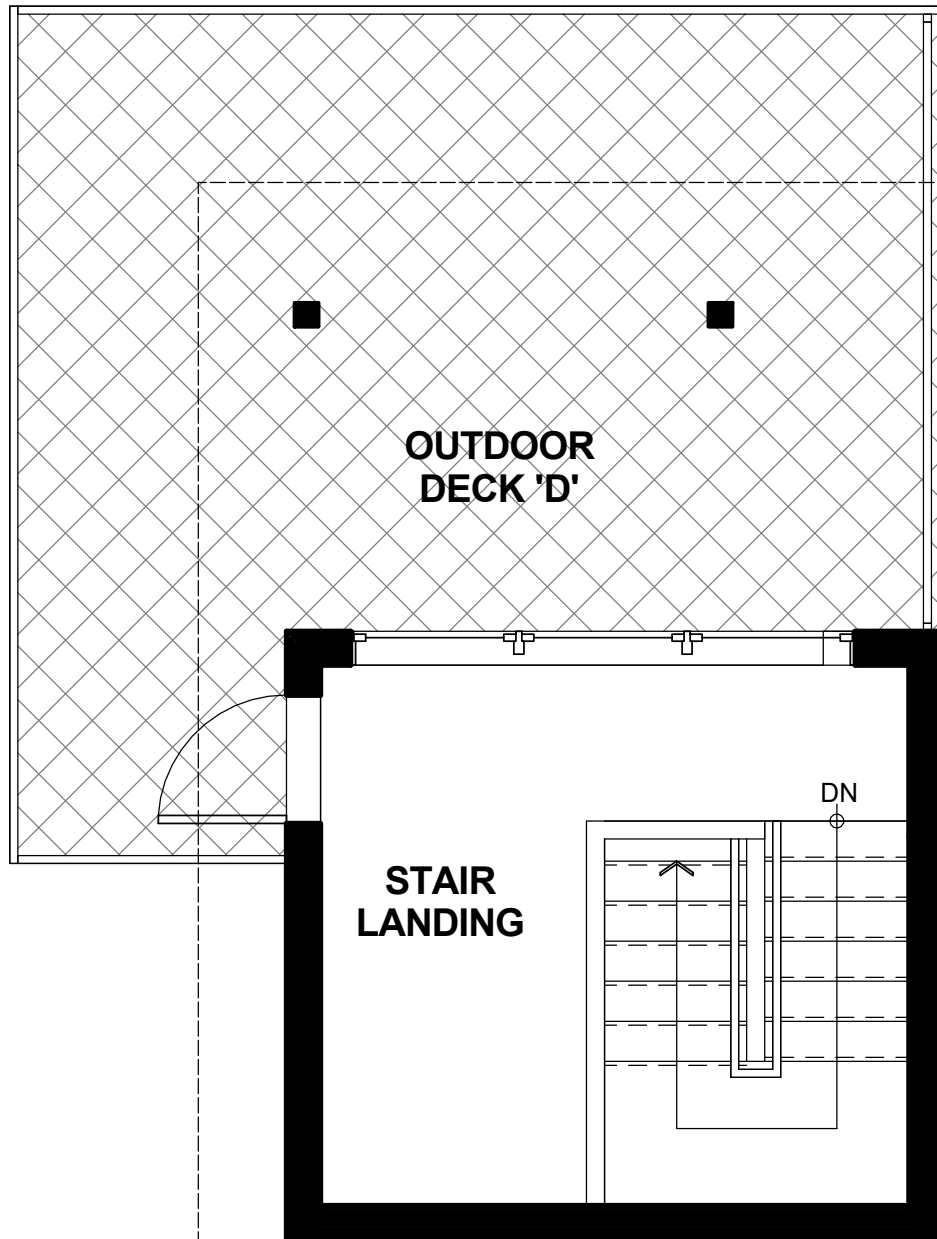
THIRD - D Scale 1/4" = 1'- 0"
